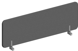
KOLEKSIYON SCREEN S0 BOPF1450 Overall Width: 1450 mm / 57" Overall Depth: 22 mm / 0.8" Overall Height: 390 mm / 15.3"
