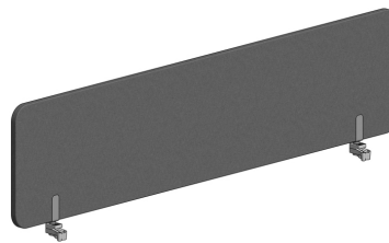
KOLEKSIYON SCREEN S0 BOPF 1650 Overall Width: 1650 mm / 64.9" Overall Depth: 22 mm / 0.8" Overall Height: 390 mm / 15.3"
