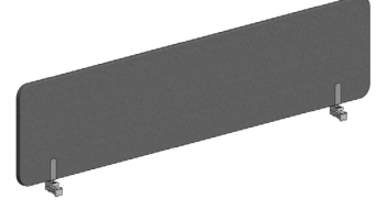
KOLEKSİYON PANEL S0 OPF1850 L: 1850 mm / 72.83 inch D: 22 mm / 0.87 inch H: 390 mm / 15.35 inch
