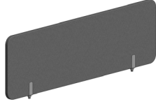
KOLEKSİYON PANEL S0 APF1250 L: 1250 mm / 49.21 inch D: 22 mm / 0.87 inch H: 390 mm / 15.35 inch
