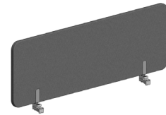
KOLEKSİYON PANEL S0 OPF1250 L: 1250 mm / 49.21 inch D: 22 mm / 0.87 inch H: 390 mm / 15.35 inch
