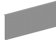
KOLEKSİYON PANEL S0 MPS1040 L: 1040 mm / 55.11 inch D: 20 mm / 0.78 inch H: 375 mm / 14.76 inch
